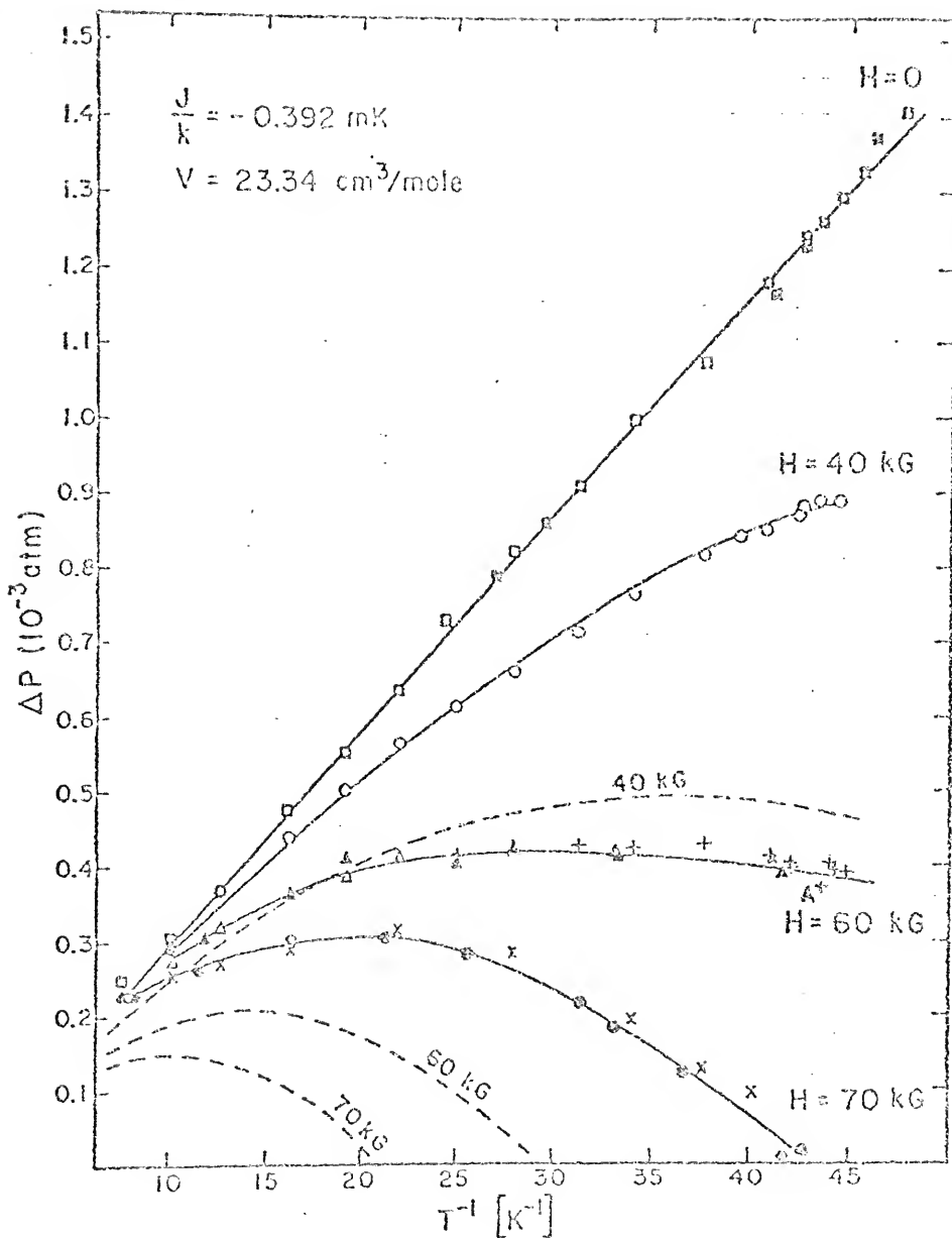
Fig. 4 High-Field Pressure Measurements. Pressure difference versus T^{-1} for v = 23.34 \text{ cm}^3/\text{mole} in several magnetic fields. The dashed curves show the calculated behavior based on the HNN model, equation (1.11). (Note: H = B ; 1 KG = 0.1 T; 1 atm = 101.3 kPa.) (After Kirk and Adams, 1971.)
